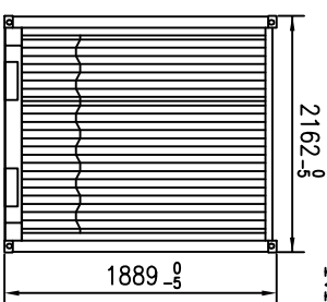
SECTION C-C 1:10
